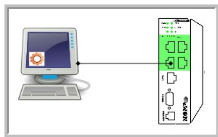
Connection through company LAN
