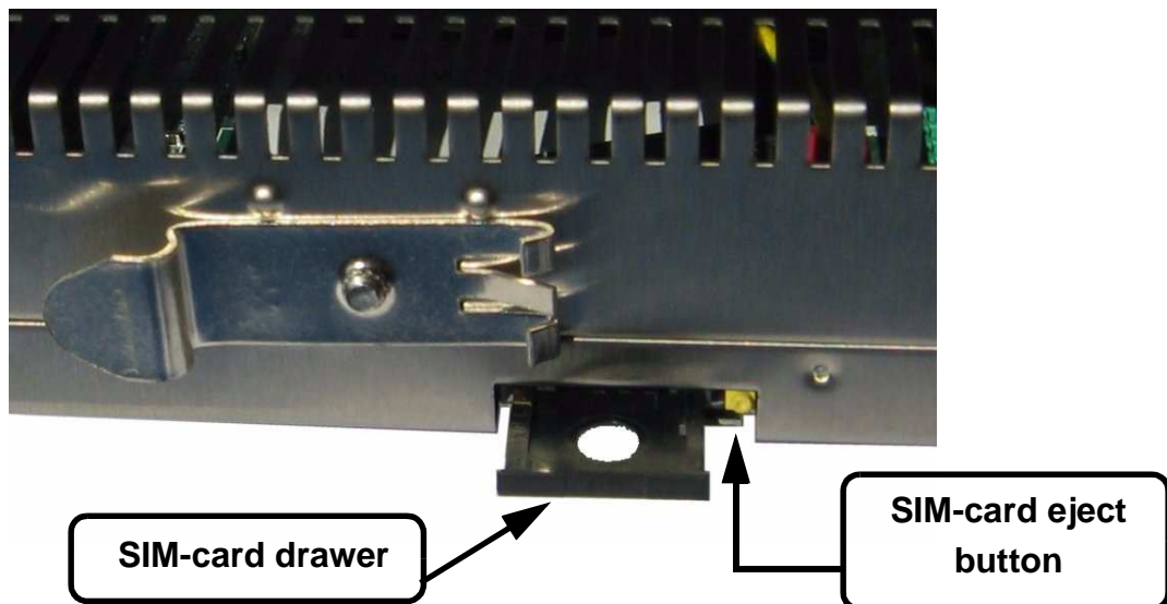
Figure 6: SIM-card insertion
