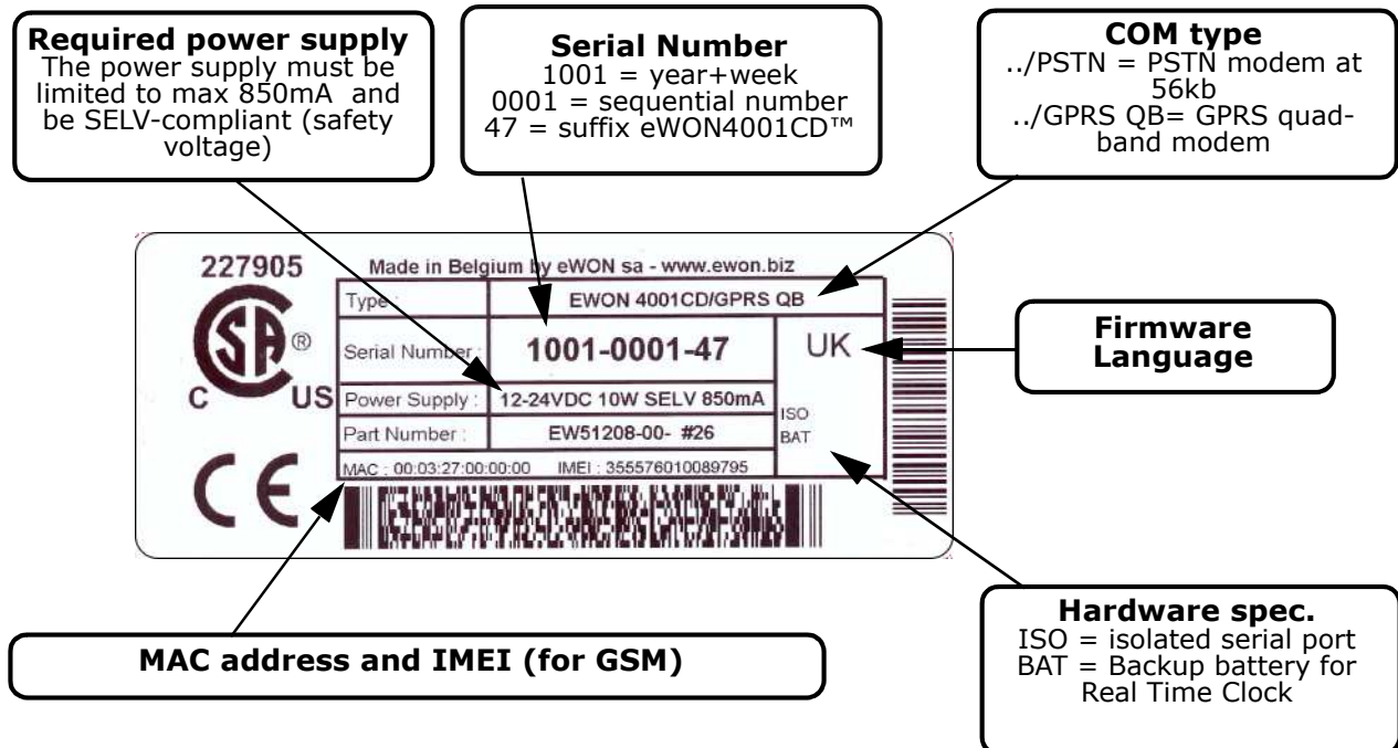
Figure 2: eWON Label
