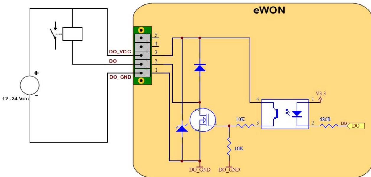
Figure 9: Digital output: wiring diagram
