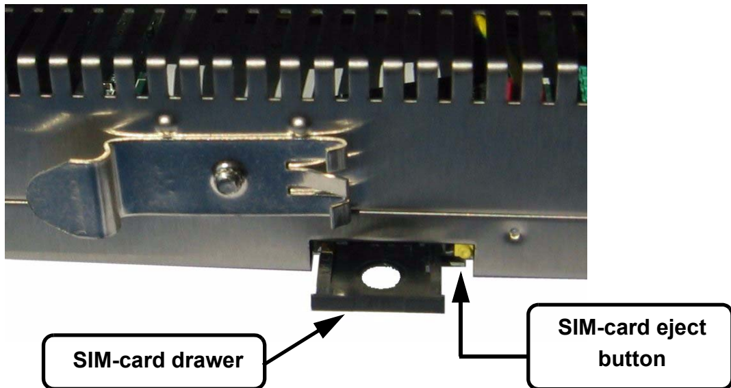
Figure 7: SIM-card insertion
