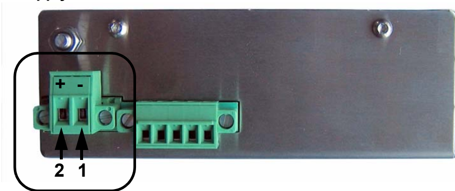
Figure 10: Power supply connector: eWON Mating female connector (included)
