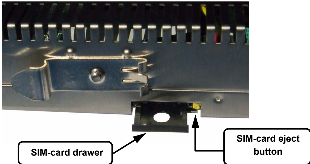
Figure 6: SIM-card insertion
