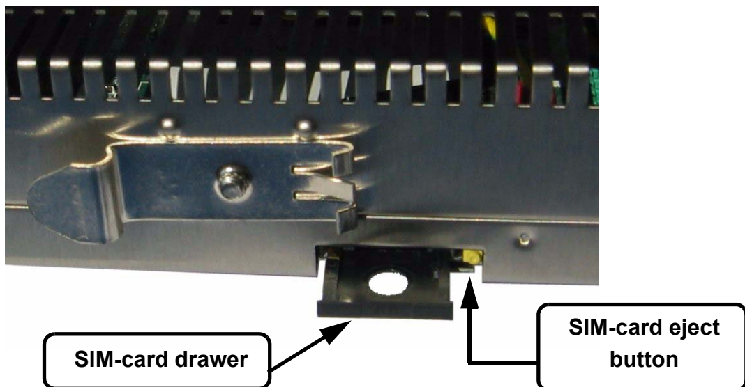
Figure 6: SIM-card insertion
